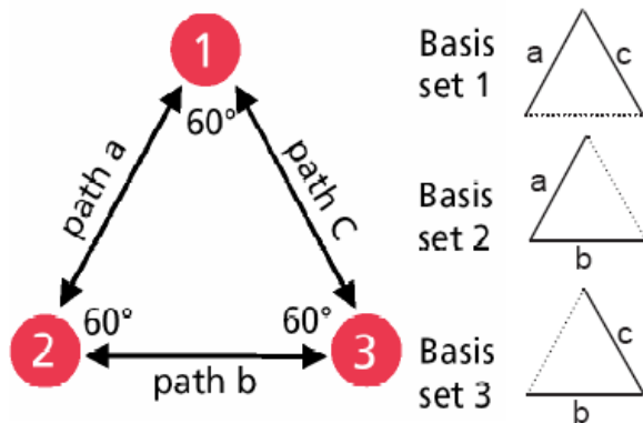
Figure 2. The equilateral triangle configuration of the three transducers provides three possible sets of basis vectors. The combinations yield bi-directional measurements on the paths labelled a, b and c. These measurements are used to determine the wind velocity components parallel to each of the three paths.
