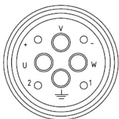
INTERCONNECTRON SIZE 1.5 8 PIN
