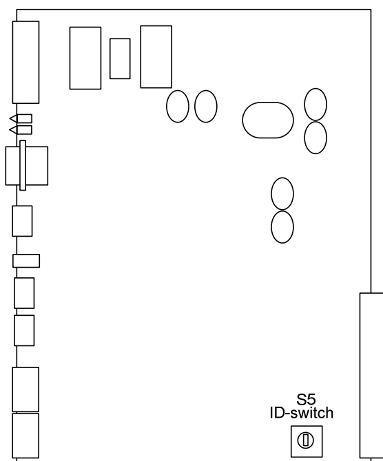
Address switch/jumpers on the PCM module
