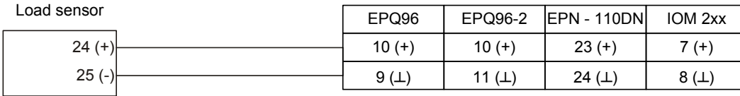
DEIF equipment terminals
