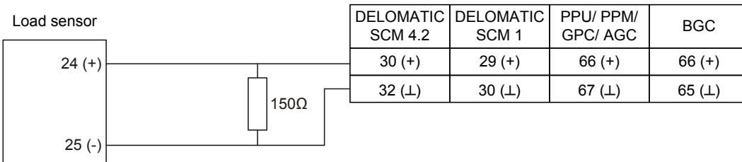
DEIF equipment terminals
