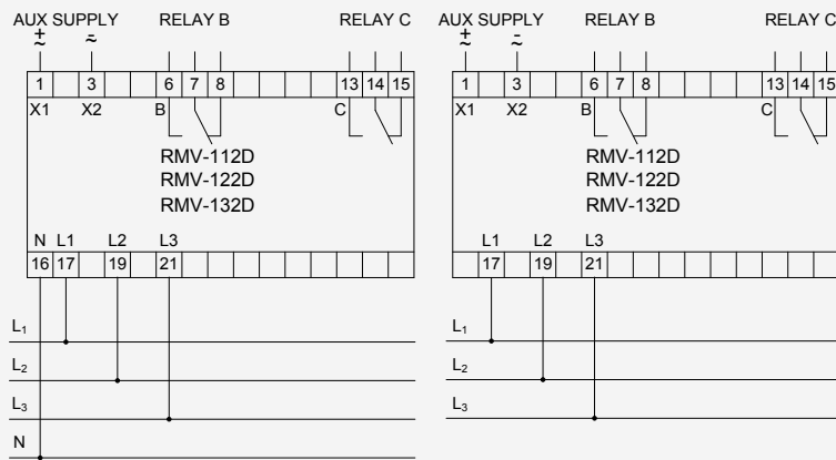
Star coupling
